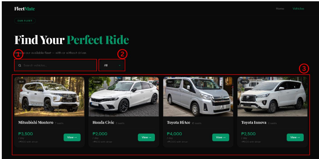
Figure 5.1 Vehicles Page
