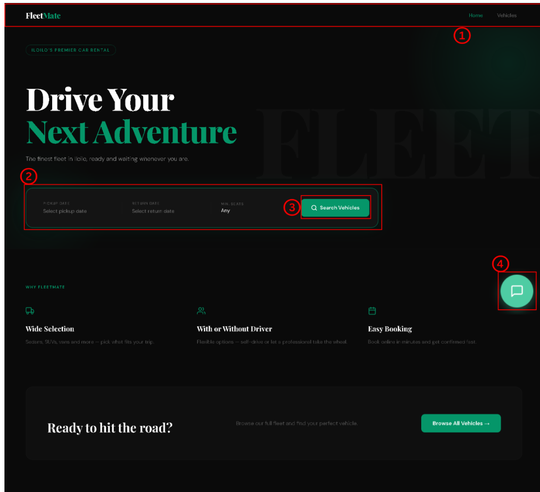
Figure 3.1 FleetMate Homepage
